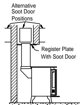
Fig. 11. Horizontal Register Plate With Optional Vertical Rear Flue Connector
